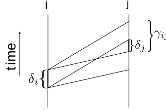
Fig. 1. Flexibility for the events i and j . By increasing the flexibility \delta_i , the flexibility for the connected node will be reduced by the same amount such that the sum of both values is at most the arc span \gamma_{ij} .
