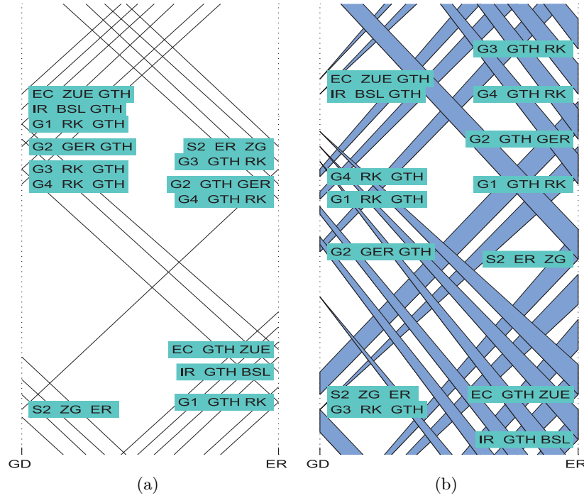
Fig. 4. (a) The generated timetable without event slots from the 2007 SBB service intention visualized in a time-space diagram. The horizontal axis represents the route from Arth-Goldau (GD) towards the alps (Erstfeld, ER), whereas the vertical axis represents the time. (b) When using event slots, each event gets an event time \pi_i and a flexibility \delta_i . In this diagram, the earliest possible line and the latest possible line are filled in grey. Any choice for train trajectories in the grey zones are feasible from the macro scheduling point of view.
