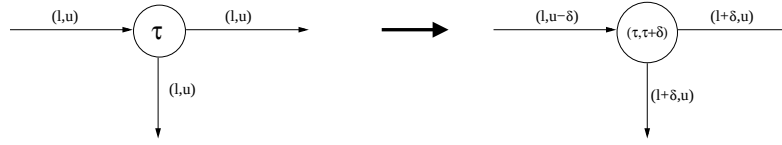
Fig. 2. Introducing an event slot of size \delta_i at event i leads to adapted constraint bounds in the PESP graph. The upper bound of incoming constraints is reduced by \delta_i and the lower bound of outgoing arcs is increased by \delta_i .
