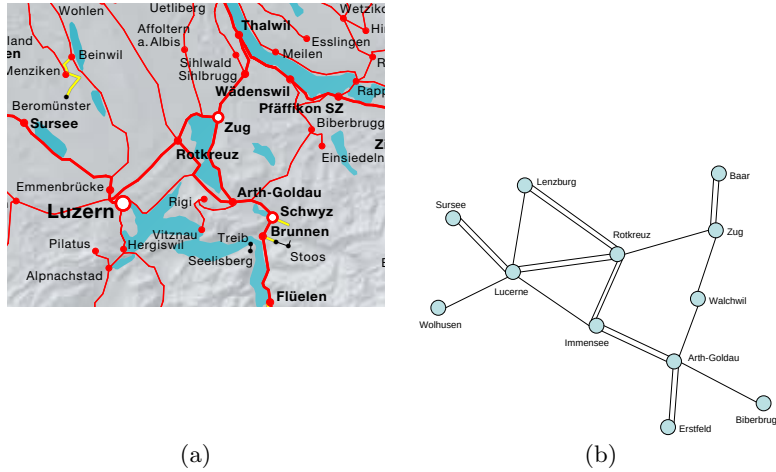
Fig. 3. (a) The test case region connecting the towns Zug – Lucerne – Arth Goldau in central Switzerland. (b) The track topology is partly double track and partly single track and is used by regional and intercity trains as well as freight trains. All the events in the PESP model correspond to departure or arrival times at stations in this picture.
